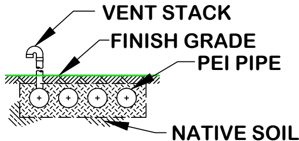
SECTION VIEW - IN GROUND
