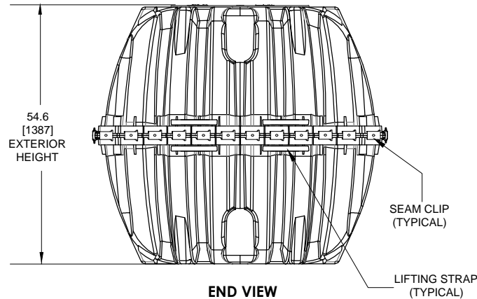
END VIEW
