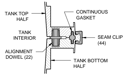
Ⓢ MID-HEIGHT SEAM SECTION DETAIL
