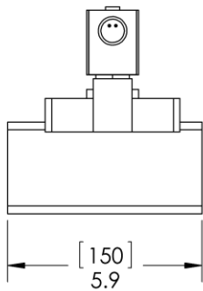
SOLENOID VALVE, NC, BRONZE 2 INCLUDED W/AUTOVALVE SYSTEM
