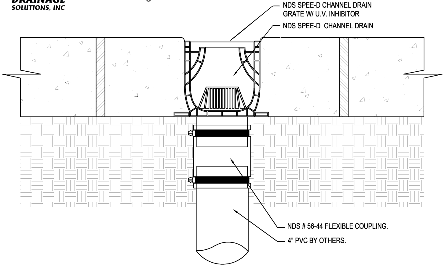
SECTION
