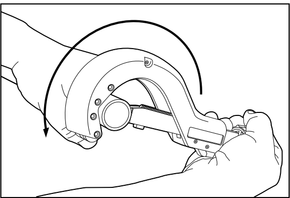
5. Depending on pipe or tubing material, tighten knob 1/4 to 3/4 turn in direction shown. Repeat tightening each revolution until cut is complete.
