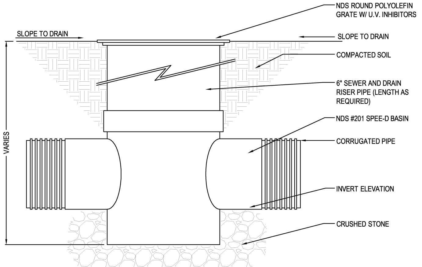
SECTION
