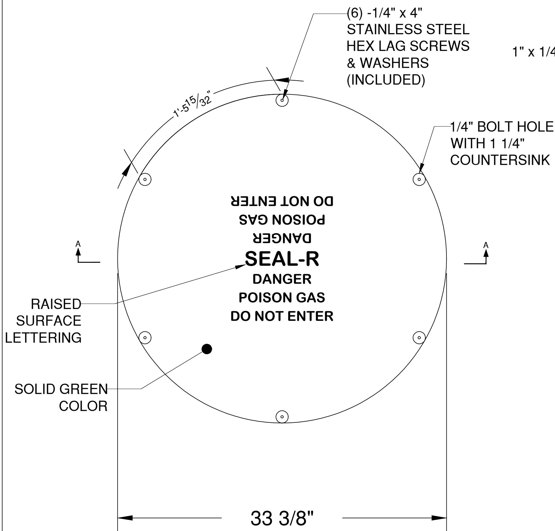
TOP VIEW
