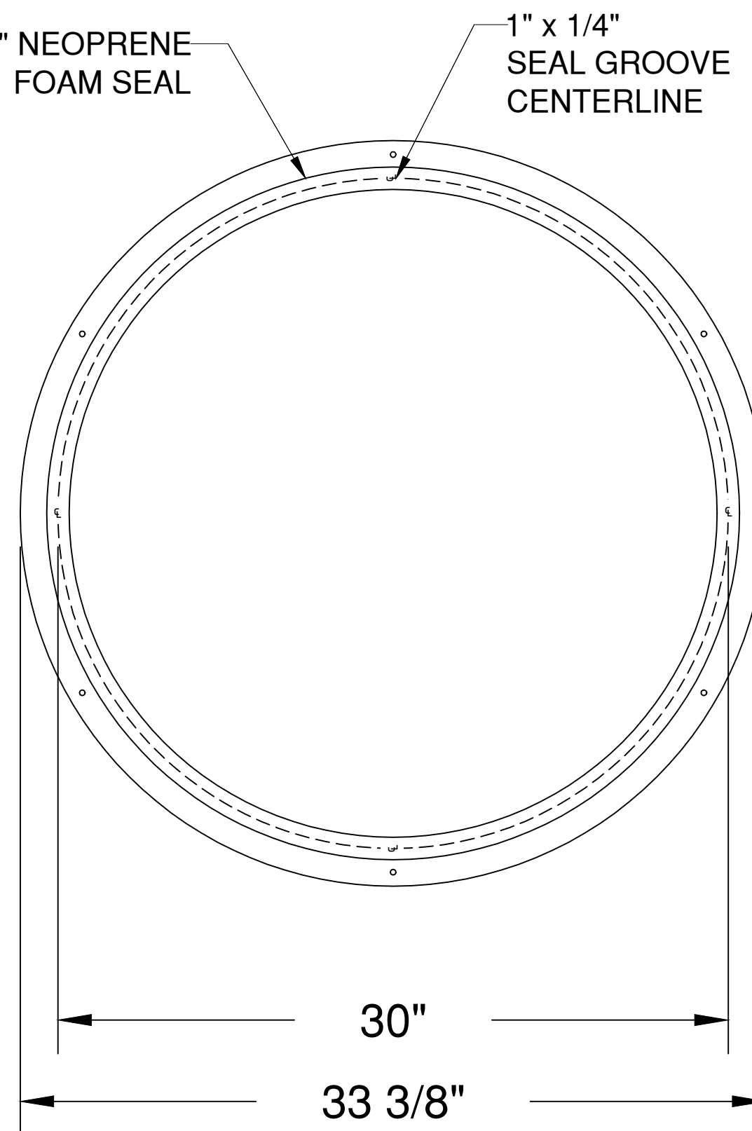
BOTTOM VIEW
