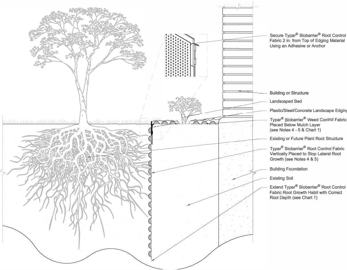
Biobarrier® : Foundation Protection Application Scale : N.T.S.
