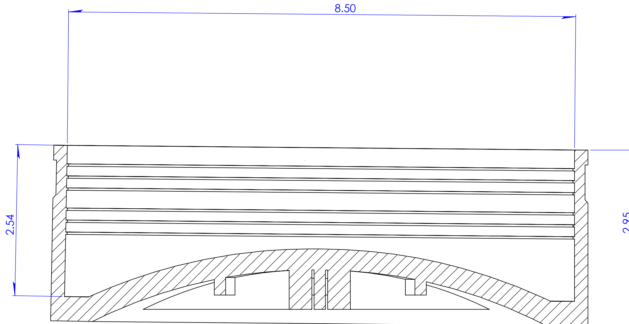
SECTION B-B SCALE 1 : 1
