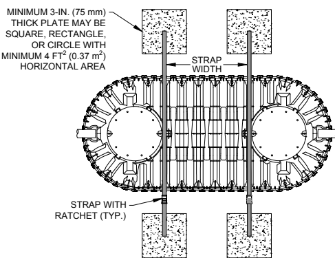
Figure 8: Precast Concrete Plate Anchor Ballast Options
