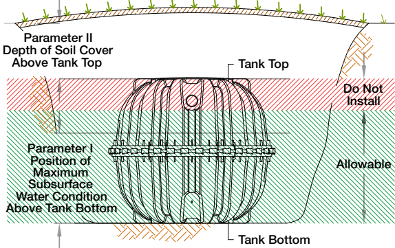
Figure 2: Buoyancy Control Parameters for Table 1
