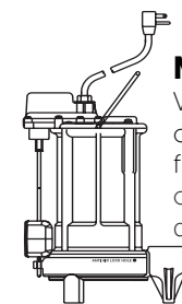
Model 253 Wide-angle float switch with series (piggyback) plug, allows manual operation of pump
