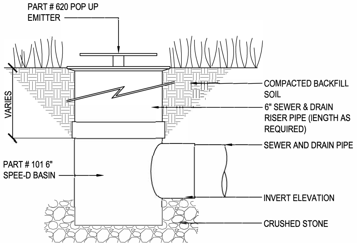
SECTION
