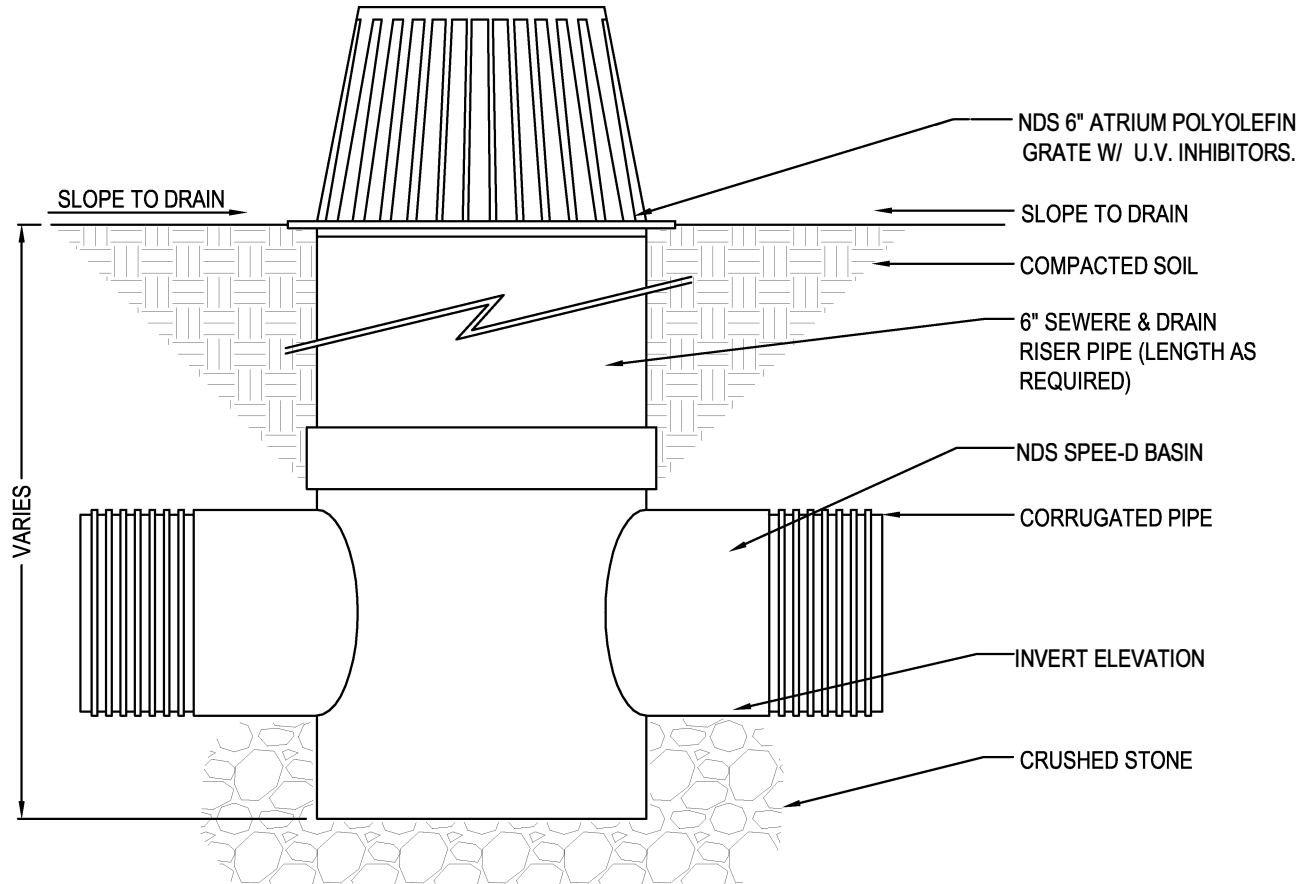
SECTION
