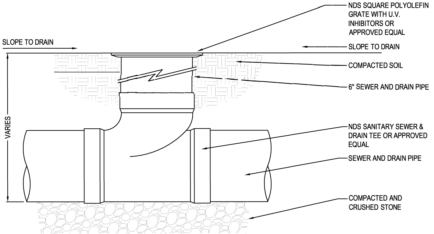
SECTION
