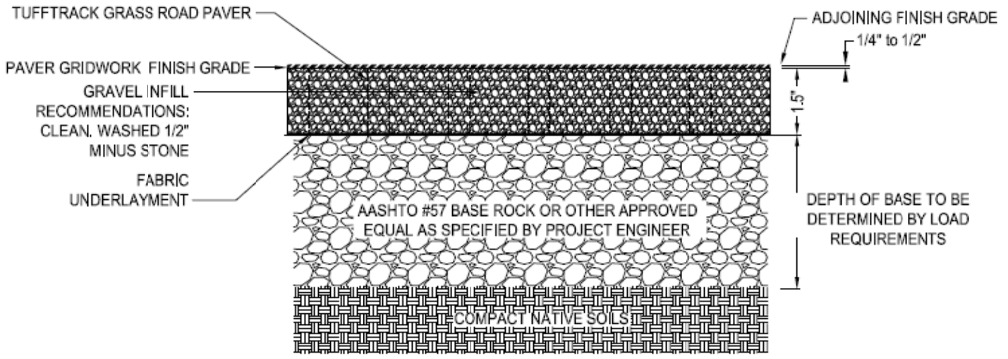
SECTION
